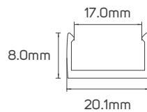
611791 - PVC Profile
